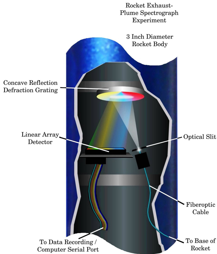
Figure 4. Cutaway diagram of custom-built spectrometer in avionics bay.
