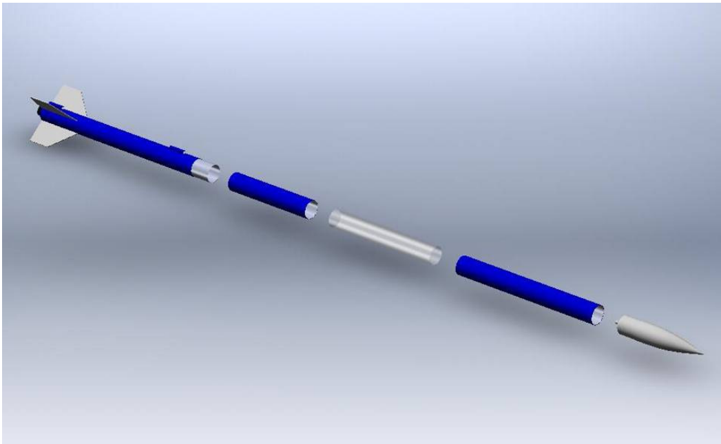
Figure 3. SolidWorks representation of flight vehicle. The aft tube houses the 36" motor mount. The middle tubes house the electronics, and the forward tube houses the parachutes.
